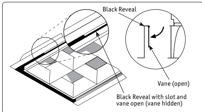
AIR WITH VANES (SUPPLY/RETURN OPTIONS)
