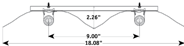
2-Lamp Cross Section
