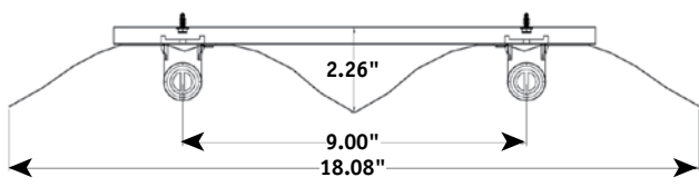
2-Lamp Cross Section
