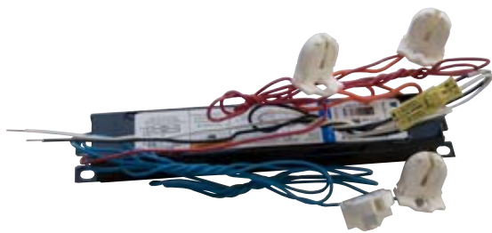
(1) Pre-wired Ballast
