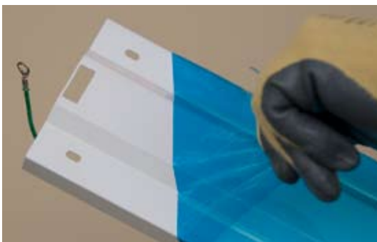
5. Remove protective film from Ballast Cover .
